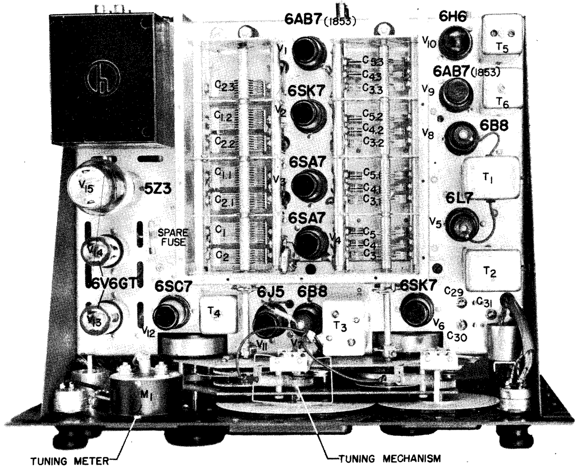
FIG. 9—SX28-A—REAR VIEW
