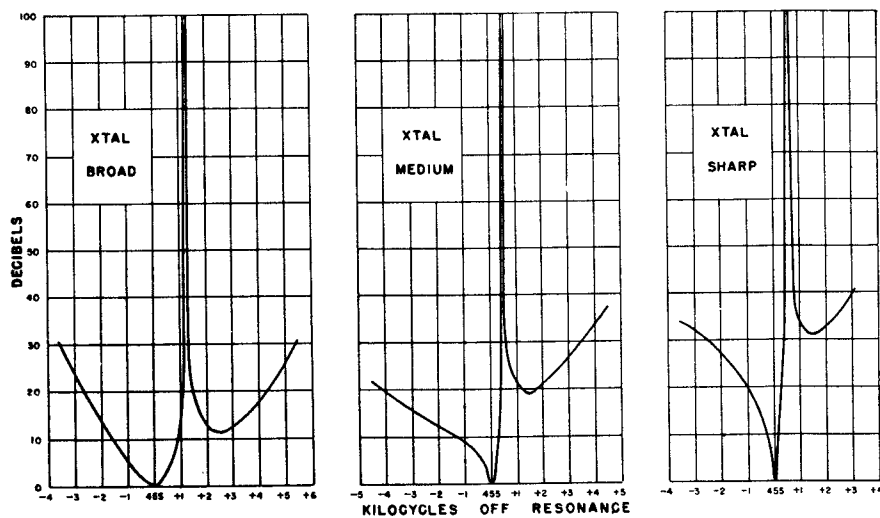
FIG. 4—CRYSTAL SELECTIVITY
